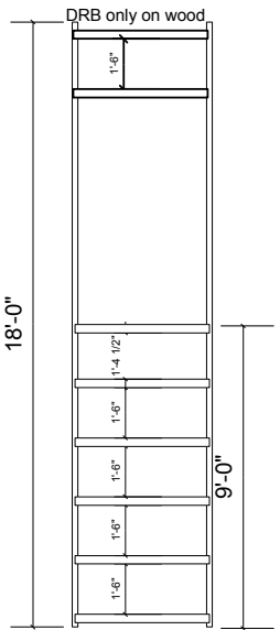
walkway Section
